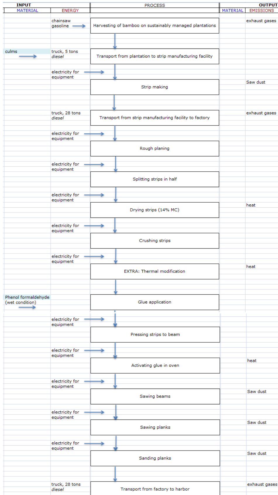
Flowchart for the production of Bamboo X-treme
